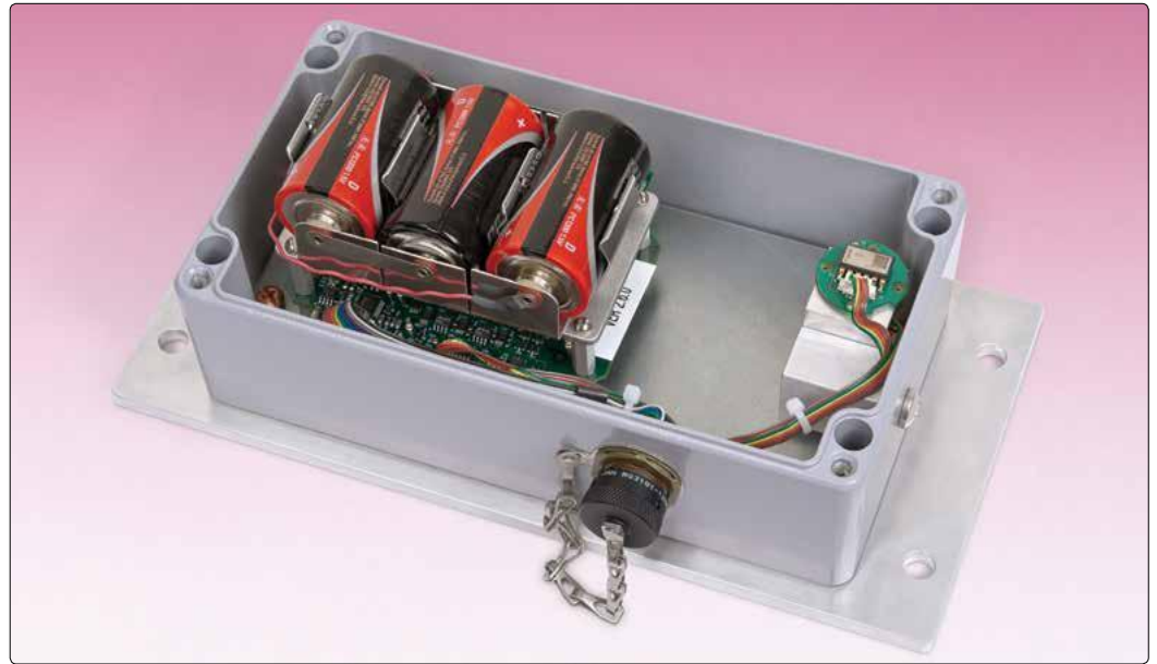
● Model 8003C-2 MEMS Datalogger shown with cover removed.
