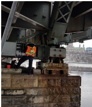
Installation of data acquisition systems under the Alexandra bridge.
