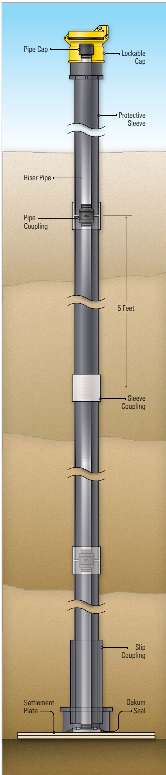
Model 4625 used to monitor settlement on an existing ground surface, after the placement of an embankment. Shown with protective PVC sleeve.
