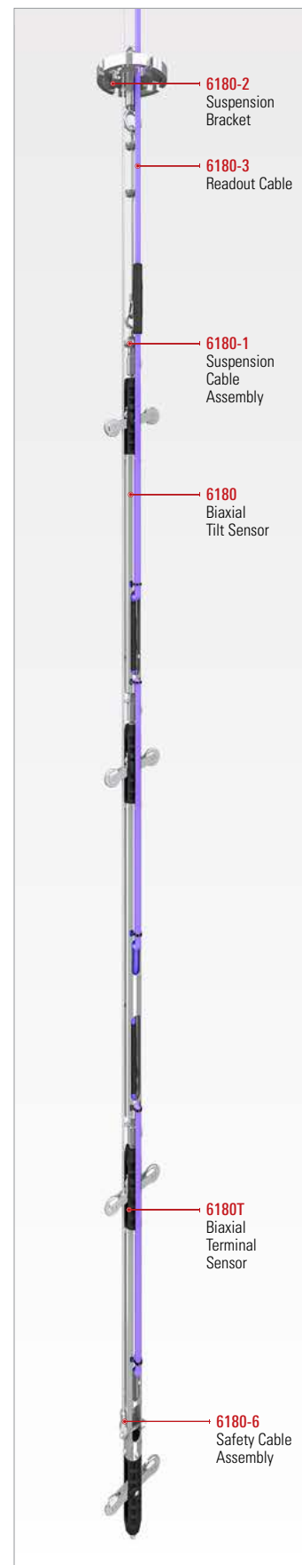
Model 6180 Vertical In-Place Inclinometer.
