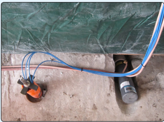
• In-place inclinometer and inclined multiple-point borehole extensometer underneath the McKenzie Tower
